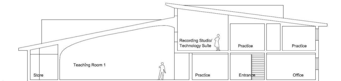
CROSS SECTION
